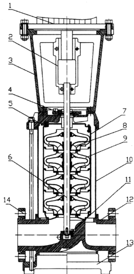
65GDLF32 - 100GDLF90
