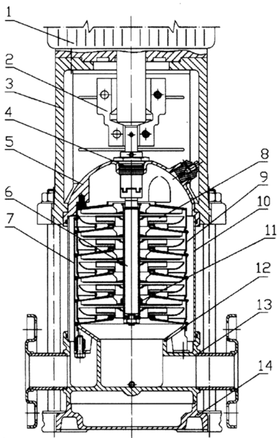
40GDLF8 - 50GDLF20
